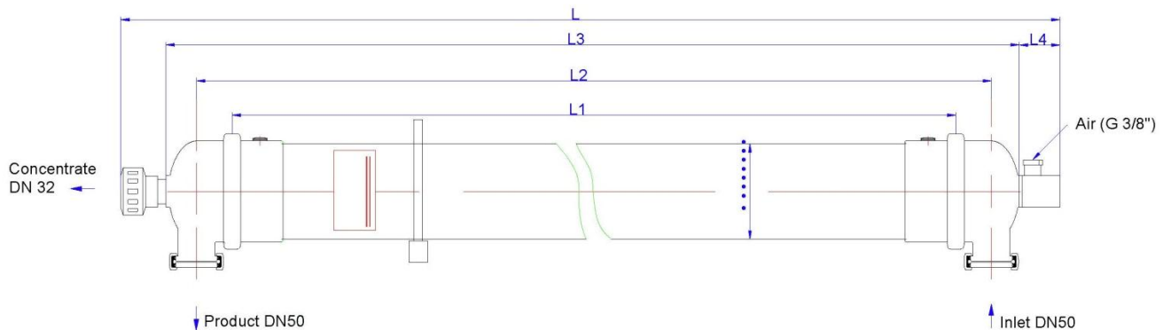
Figure 1: SFP and SFD 2660 (6-inch diameter)
